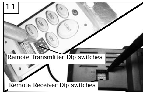
11 Set dip switches on the Remote Transmitter and Remote Receiver to the same settings. This must be done so the units will communicate properly. If you have other fans you can set to control from one transmitter by setting both receivers the same as the transmitter. If you have more than one fan with remote. You can set the dip switches to different positions to have separate control.
